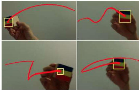
Figure 4. Kinematic characteristics.
