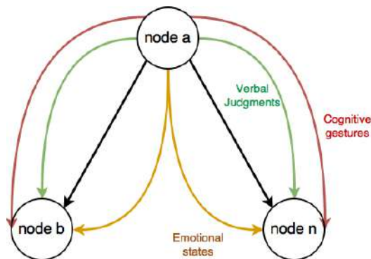
Figure 3. Graph characteristics.
